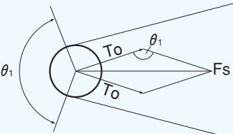
Initial tension T_o (Unit: N)
