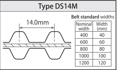
Belt size (Type DS14M)
