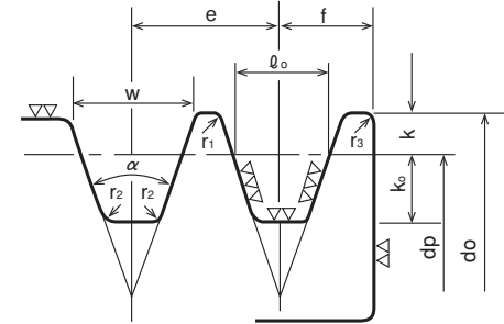
Fig. 1 Pulley groove cross section
