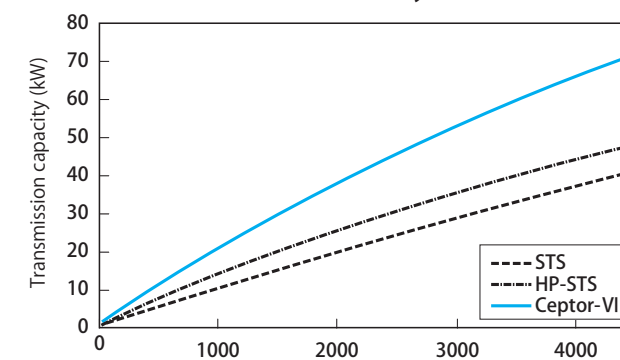
Belt width: 60 mm / Pulley: 26 teeth (S8M)
