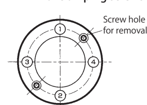
Fig. 1 Order of tightening of clamping screws
