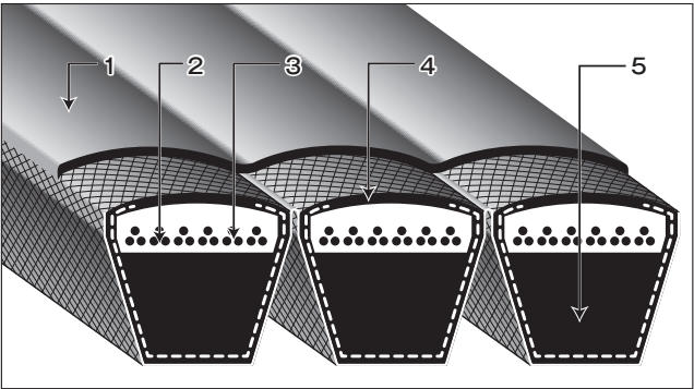
1. Tie band 2. High-elasticity aramid cord 3. Adhesion rubber 4. Cover fabric 5. Compression rubber
