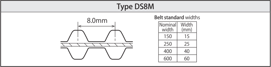
Belt size (Type DS8M)
