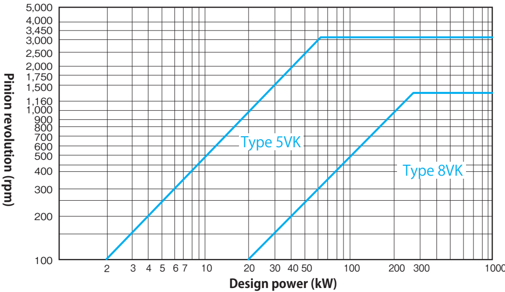
Fig. 1-4 Belt type selection diagram (Rib-Ace 2)
