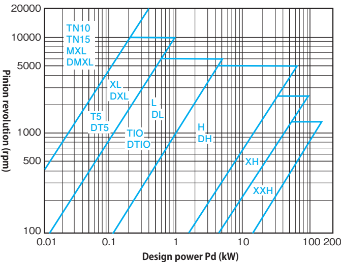
Fig. 3-5 Belt type selection diagram (Synchronous Belt)
