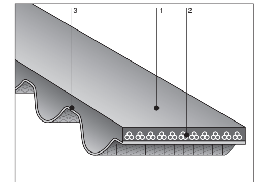
1. Rubber 2. Cord 3. Facing fabric
